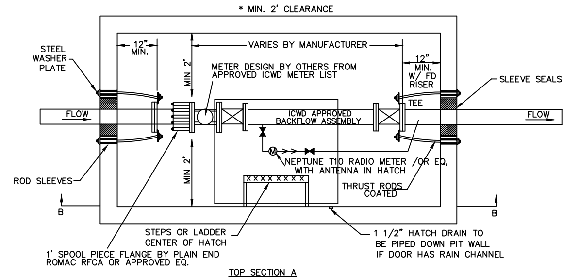
TOP SECTION A
